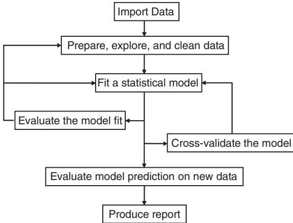
Figure 1.1 Steps in a typical data analysis
